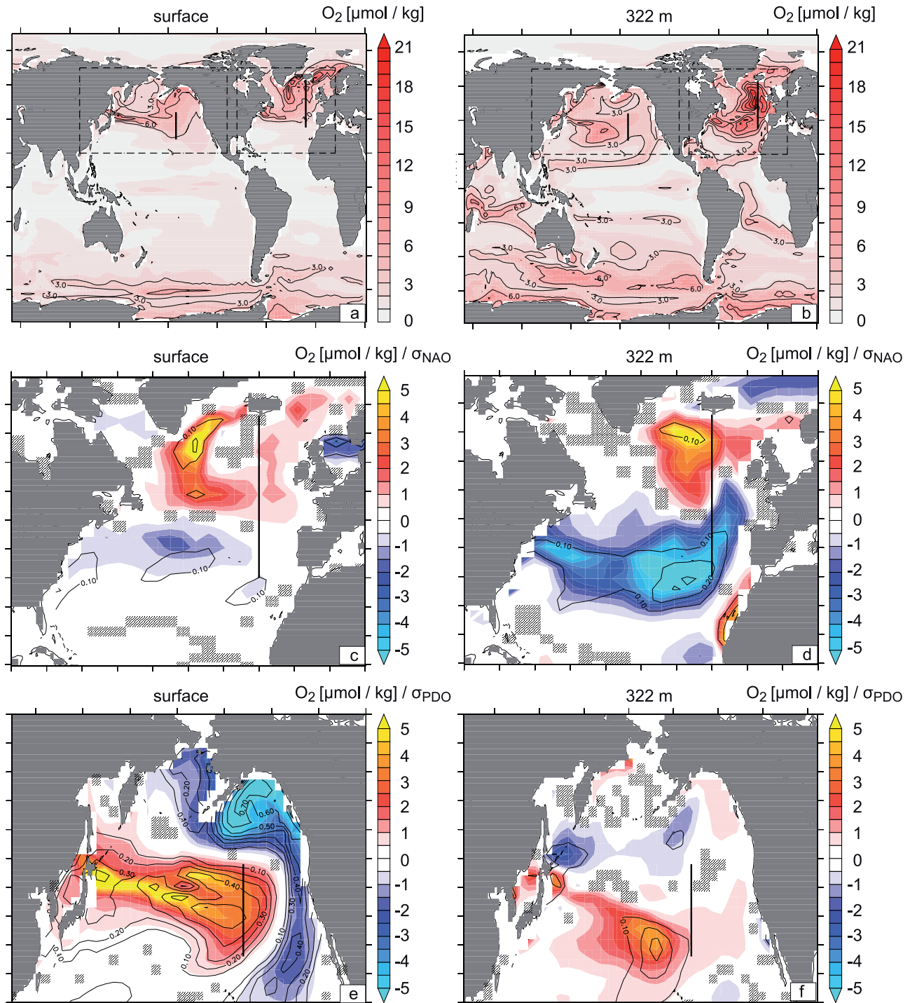
Figure 3. Internal variability in O 2 , displayed as one standard deviation of annual mean O 2 from the control simulation, (a) at surface and (b) at 322 m depth. Contours are every 3 μmol kg -1 and dashed lines show the two areas for Figures 3c–3d and 3e–3f, respectively. Regression of winter mean (October–March) and annual mean O 2 from the control simulation with the standardized annual NAO (Figures 3c and 3d) and PDO (Figures 3e and 3f) index, respectively, at (c and e) the surface and at (d and f) 322 m depth. Regression slopes correspond to one standard deviation change in the NAO and PDO index, respectively. Contour lines denote the respective squared correlation coefficients and areas without shading show statistically significant areas ( t test, p value < 0.05). Solid thick lines show the World Ocean Circulation Experiment (WOCE) A16N and WOCE P16N section.
