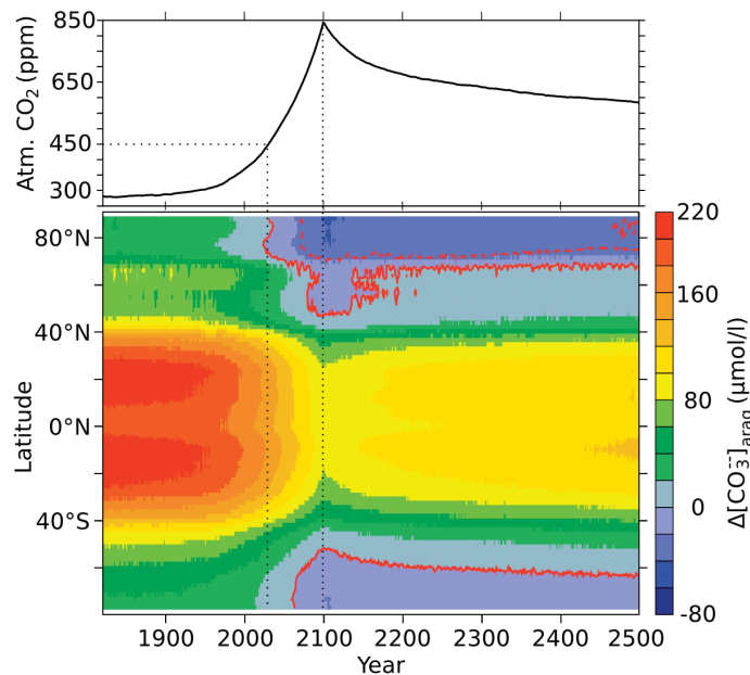
Figure 1: Simulated evolution of atmospheric CO 2 and of zonal, annual mean surface carbonate ion concentration, shown as deviation from the saturation concentration with respect to aragonite. Red lines indicate the transitions from over- to undersaturation with respect to aragonite (solid) and calcite (dashed).
