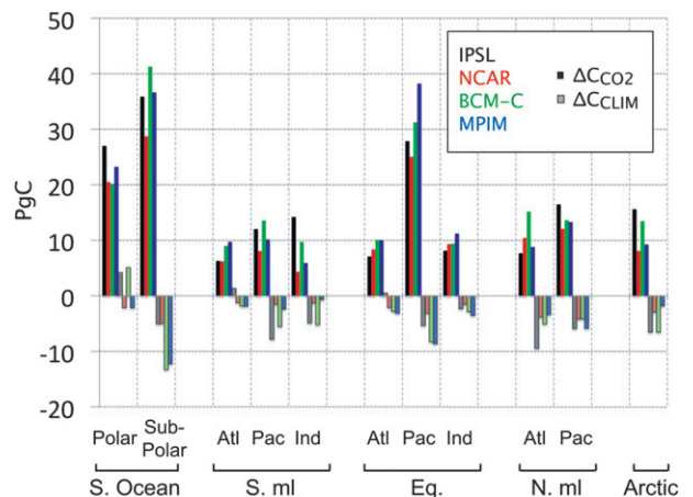
FIG. 5. Regionally integrated cumulated CO 2 uptake (PgC) to the end of this century (2010–2100) in the C 4 Ms. Here, \Delta C_{\text{CO}_2} (PgC) is represented by the strong color bars, and \Delta C_{\text{CLIM}} (PgC) is represented by the pale color bars. The coordinates of the regions are identical to Mikaloff-Fletcher et al. (2006): Southern Ocean (S. Ocean; Polar, >58°S; Subpolar, 44°–58°S), Southern midlatitudes (S. ml; 18°–44°S), equatorial (Eq.; 18°S–18°N), Northern midlatitudes (N. ml; 18°–49°N), and Arctic (>49°N).
